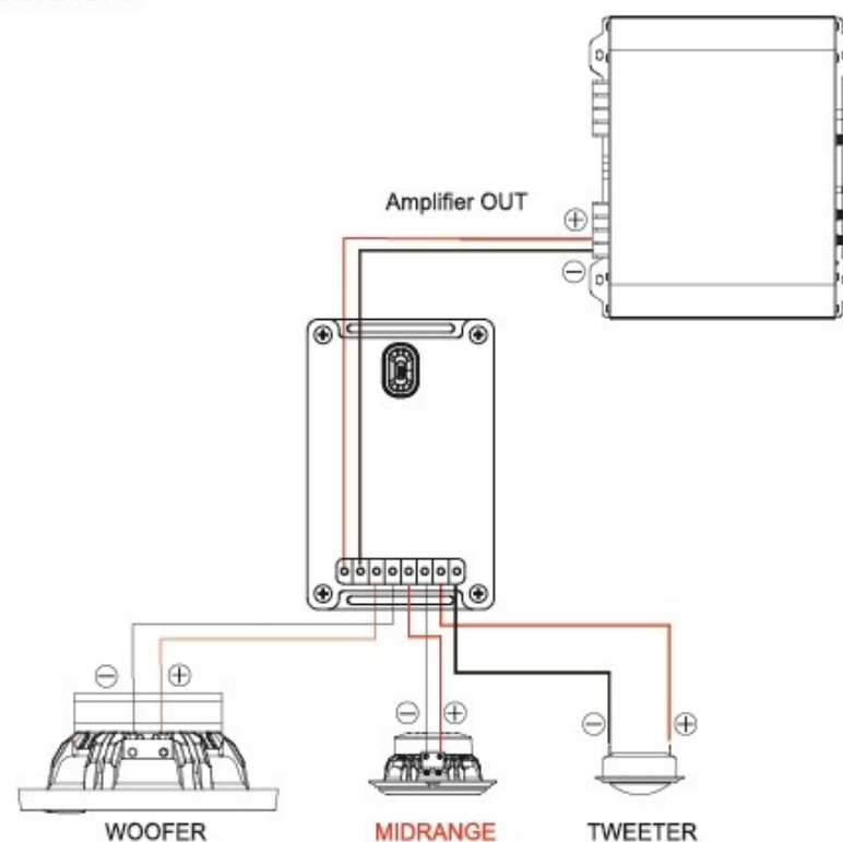
Model M7701 PASSIVE SET UP
